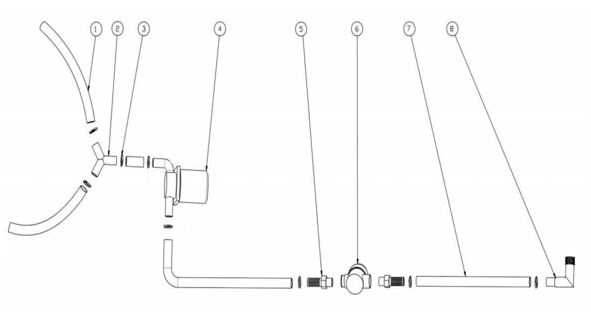
Fig. 10 -HOSE GROUP
