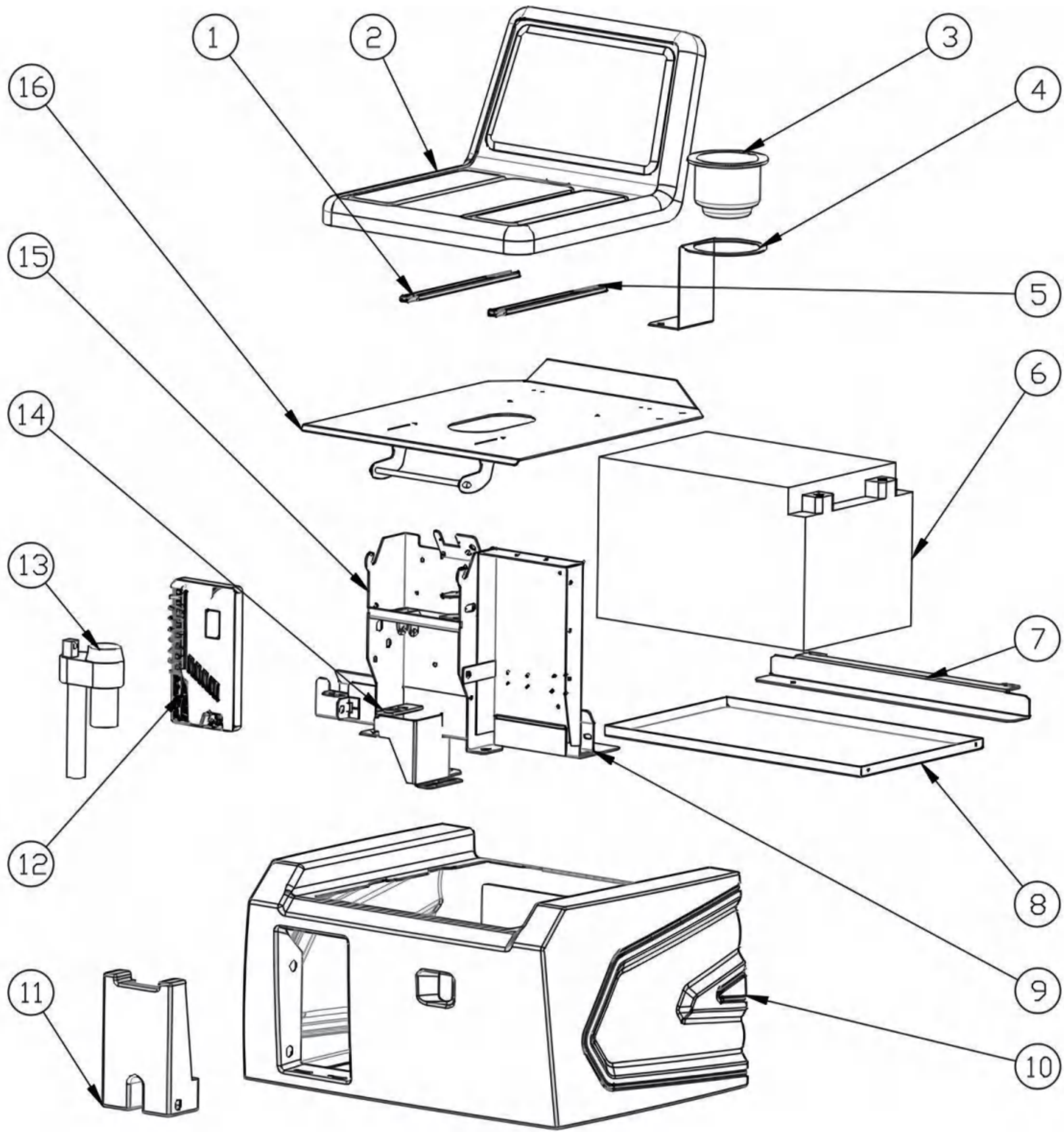
Fig. 5 -SEAT GROUP
